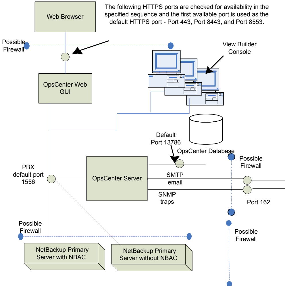
Figure 3-1 Key OpsCenter components and how they communicate
