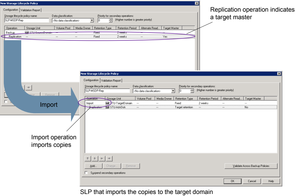
Figure 5-3 Storage lifecycle policy pair required for Auto Image Replication
