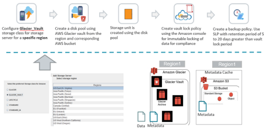
Figure 2-5 Protecting data in Amazon Glacier vault
