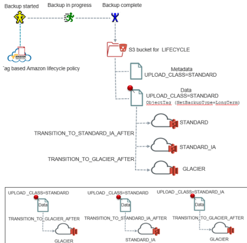
Figure 2-9 Back up process for Amazon S3 Intelligent Tiering (LIFECYCLE) storage class with possible configurations
