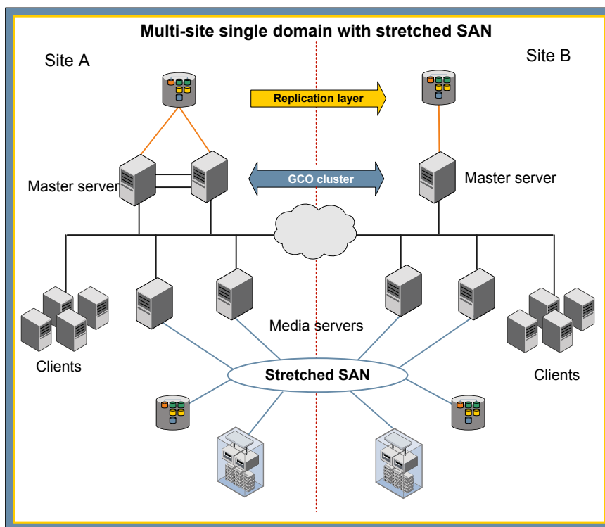
Figure 4-1 Multi-site single domain with stretched SAN
