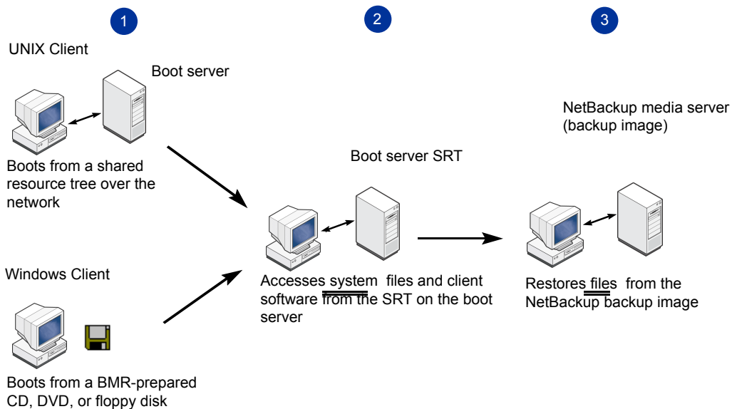
Figure 6-1 Network restore
