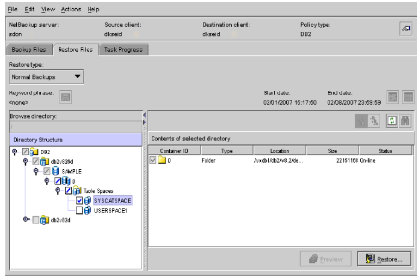
Figure 4-2 Restore window (Windows)
