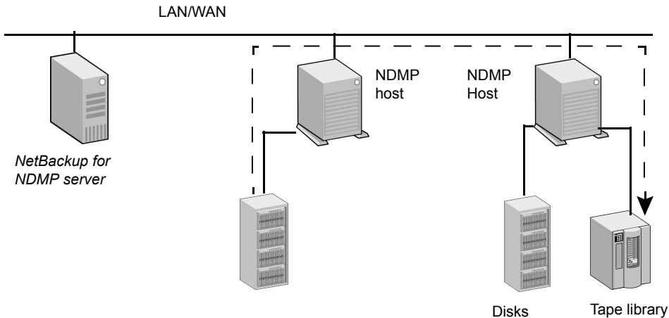
Figure 12-3 NDMP three-way backup and restore
