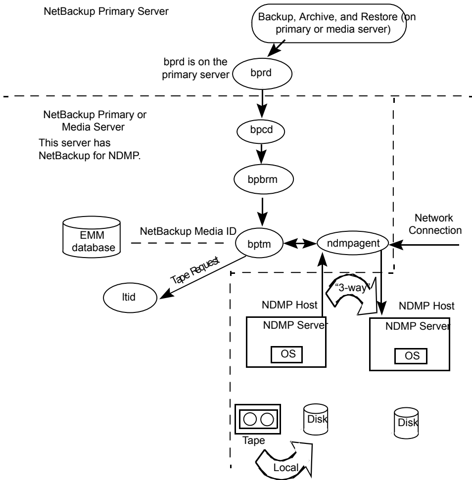
Figure 12-9 NetBackup restore processes
