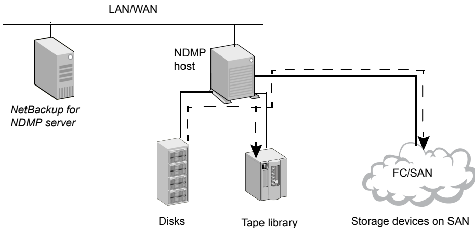
Figure 12-2 NDMP local backup and restore
