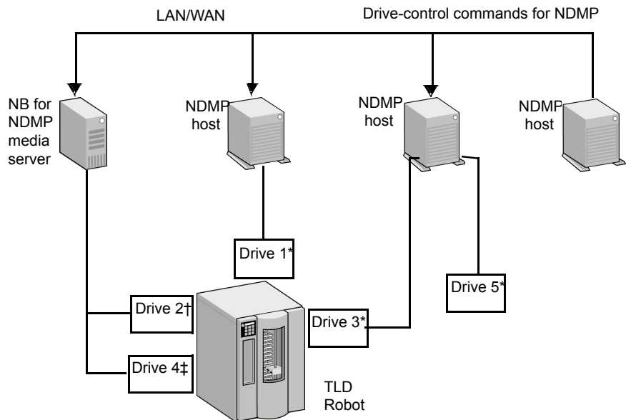
Figure 12-5 NDMP and non-NDMP storage units
