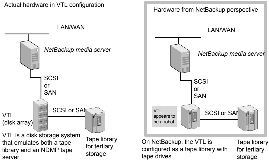
Figure 16-1 Overview of NDMP DirectCopy with VTL
