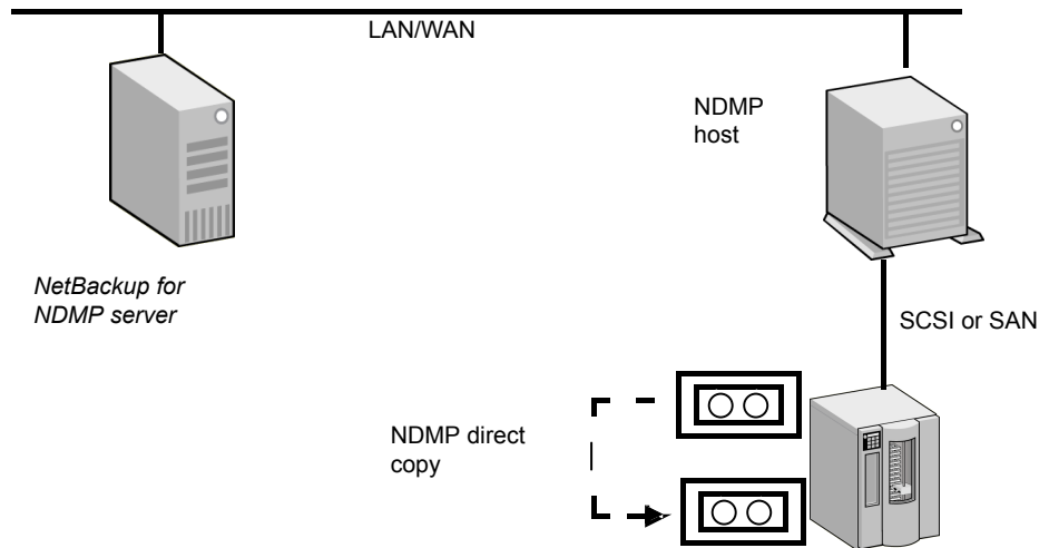
Figure 16-3 NDMP DirectCopy between tape drives accessible to an NDMP host
