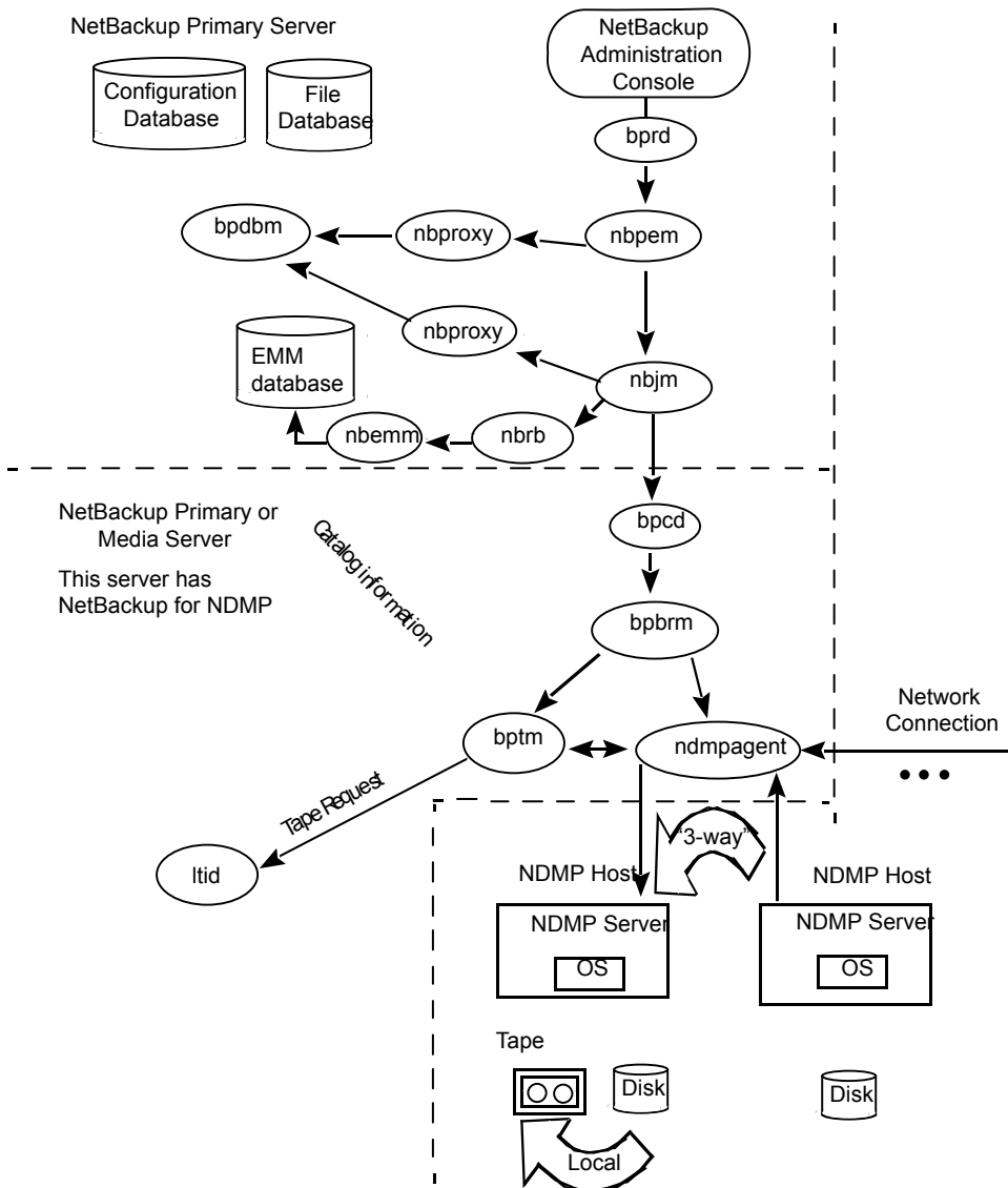
Figure 12-8 NetBackup backup processes
