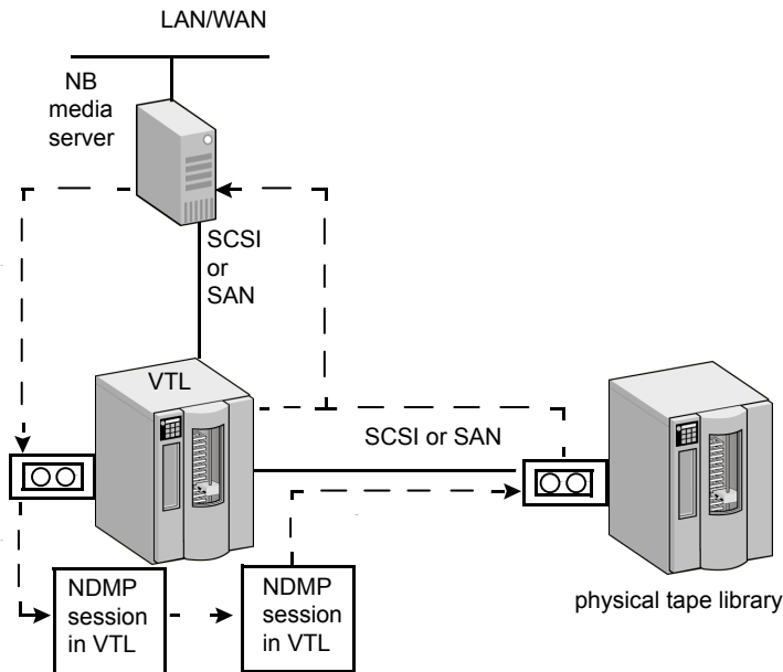
Figure 16-2 NDMP DirectCopy with VTL data flow and control
