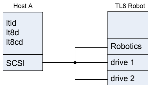
Figure A-3 Use of t18cd with single host connected to TL8 robot
