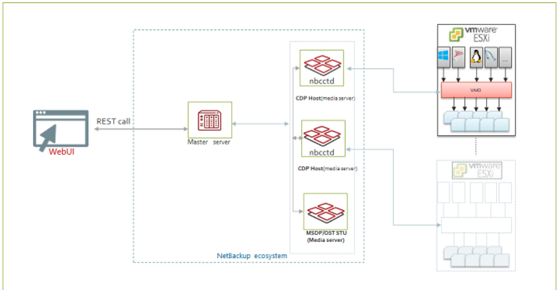
Figure 7-1 CDP architecture
