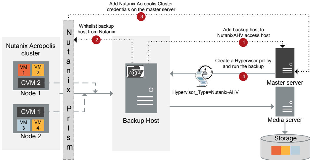
Figure 4-1 Establishing communication between NetBackup and Nutanix AHV
