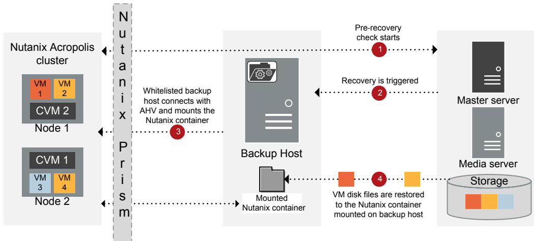
Figure 6-1 Overview of the Nutanix VM recovery process
