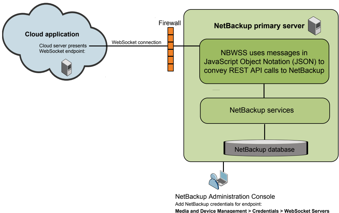
Figure 1-1 NBWSS overview
