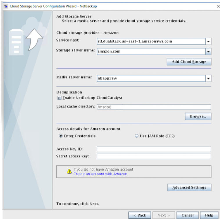
Figure 2-1 Cloud Storage Server Configuration Wizard panel for Amazon
