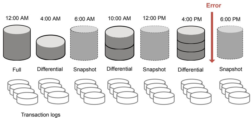
Figure 8-2 Recovering after an error when using full and copy-only backups
