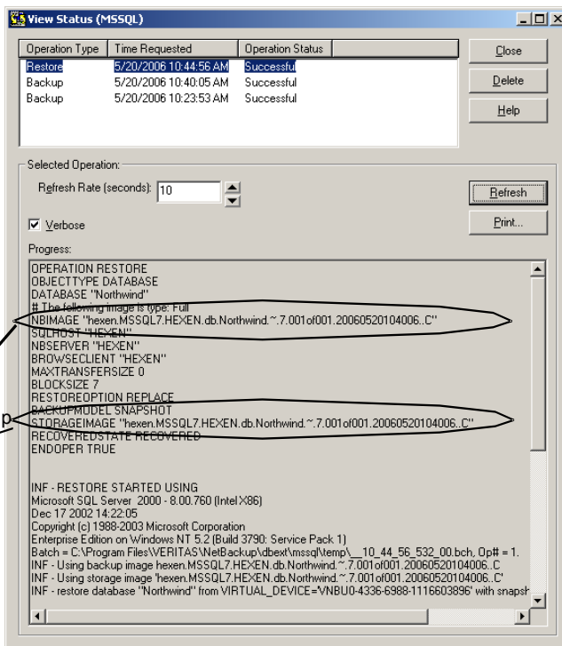
Figure 8-4 Batch file shown in the progress report for the restore operation
