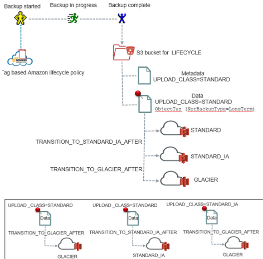
Figure 2-12 Back up process for LIFECYCLE storage class with possible configurations
