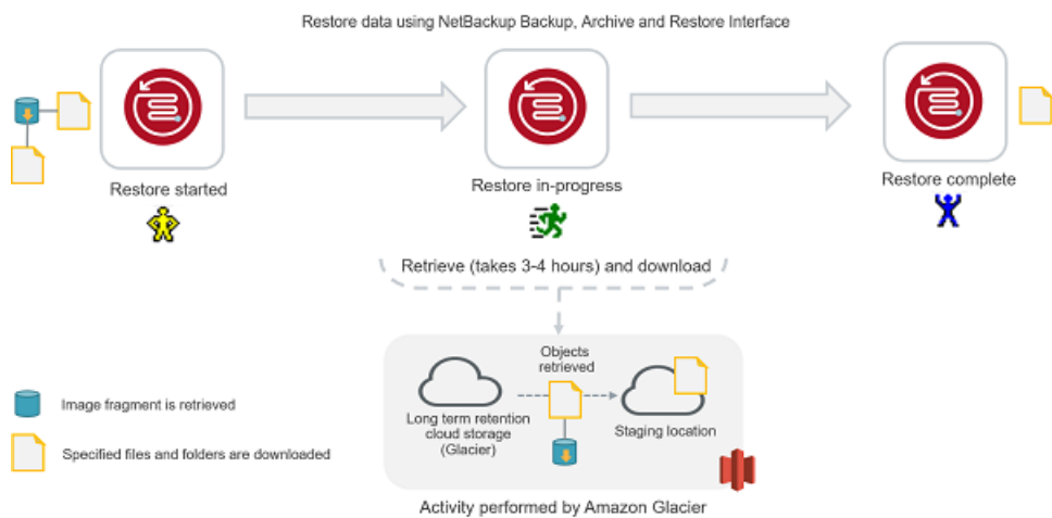
Figure 2-6 Restoring from Amazon GLACIER
