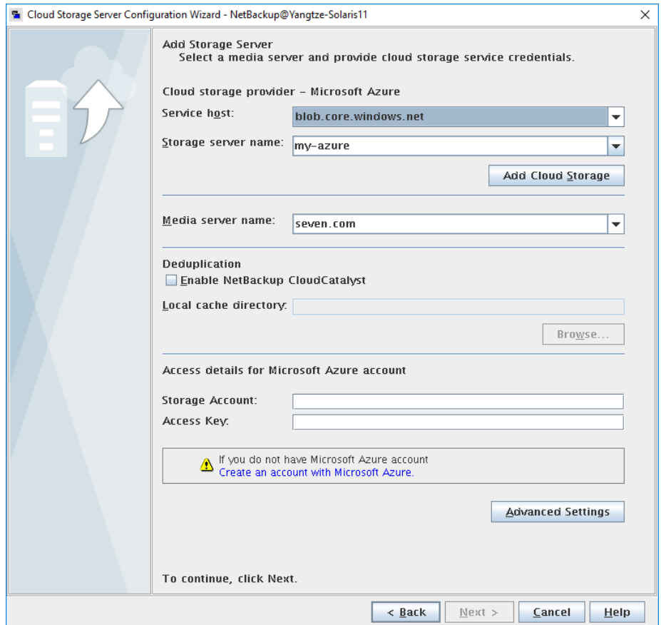
Figure 2-13 Cloud Storage Server Configuration Wizard panel for Microsoft Azure
