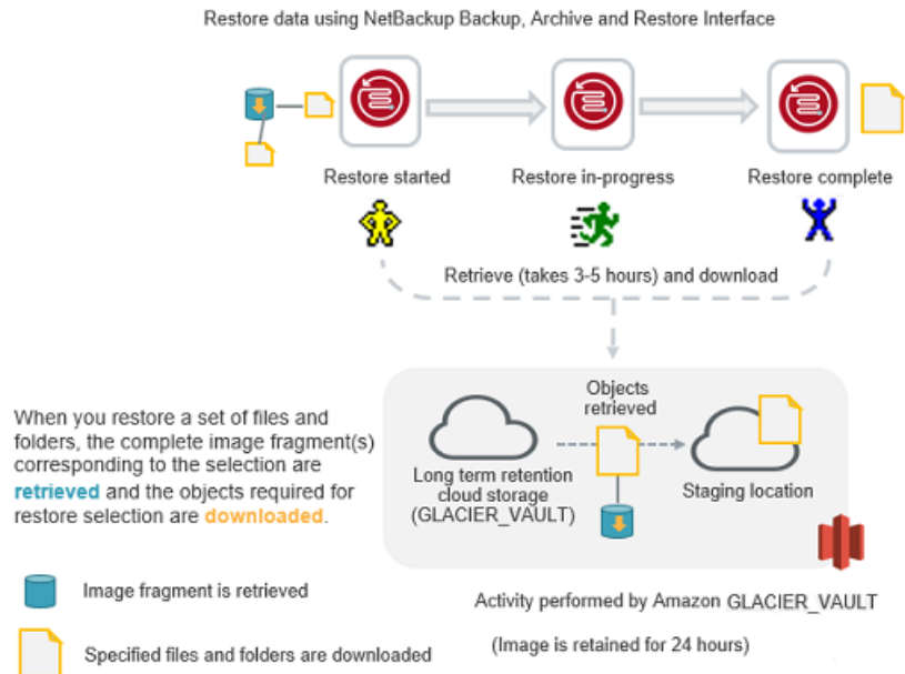
Figure 2-10 Restoring from Amazon Glacier vault
