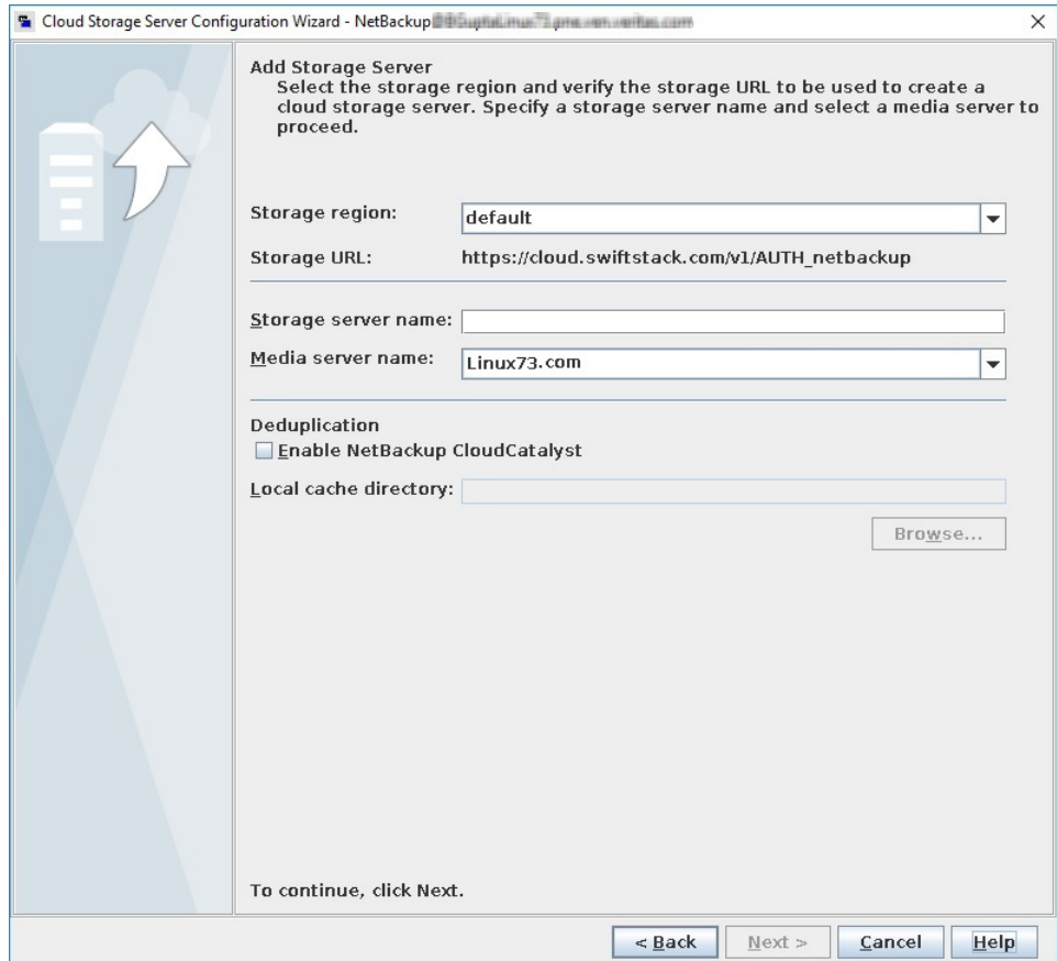
Figure 2-15 Cloud Storage Server Configuration Wizard panel
