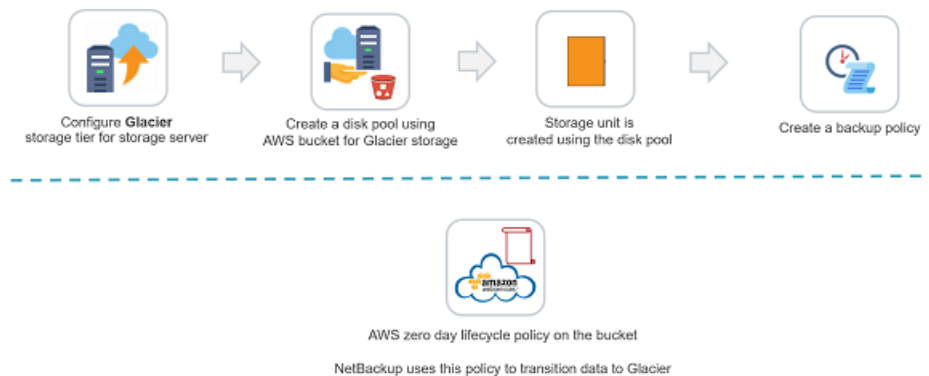
Figure 2-4 Protecting data in Amazon Glacier
