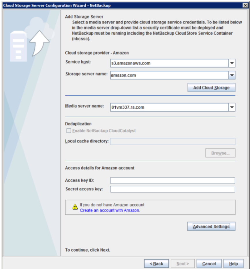
Figure 2-1 Cloud Storage Server Configuration Wizard panel for Amazon
