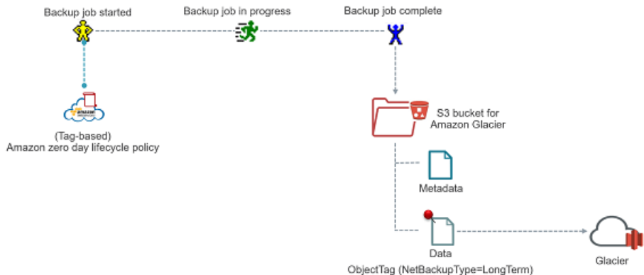
Figure 2-5 Backing up to Amazon Glacier
