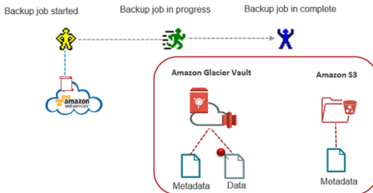
Figure 2-9 Backing up to Amazon Glacier vault
