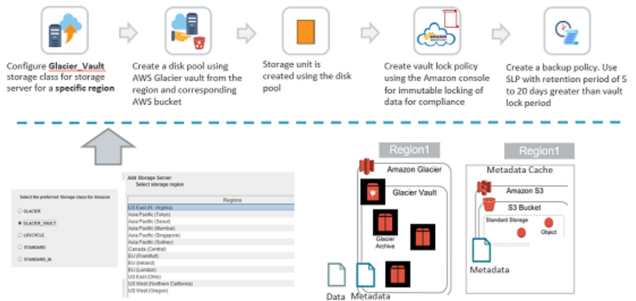
Figure 2-8 Protecting data in Amazon Glacier vault
