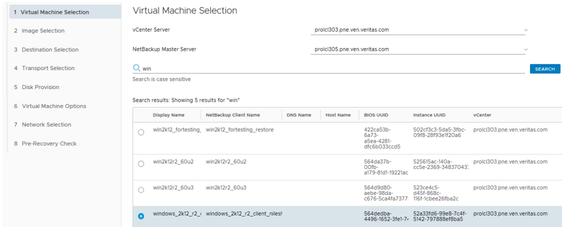
Figure 5-1 Virtual Machine Selection screen in the NetBackup Recovery Wizard for vSphere Client (HTML5)
