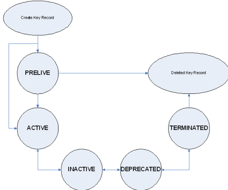
Figure 25-1 States possible for key creation
