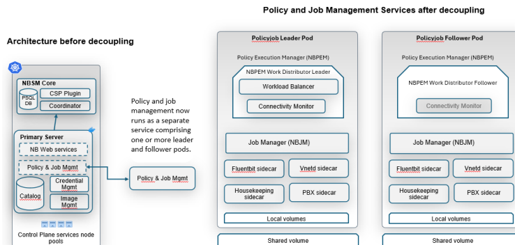
Figure 1-3 Policy and Job Management architecture
