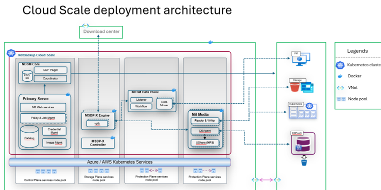
Figure 1-1 Cloud Scale architecture before decoupling
