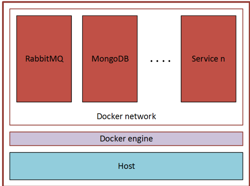
Figure 1-1 NetBackup Snapshot Manager's micro-services model
