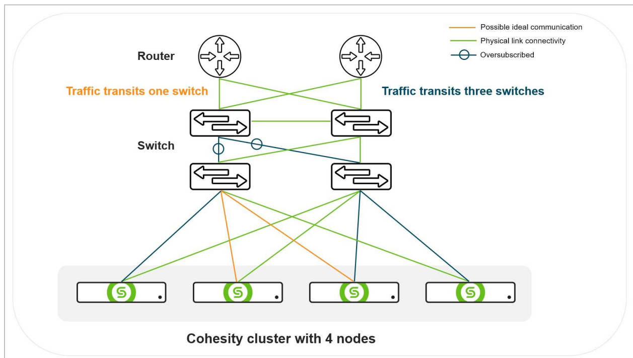
Figure 3: Cohesity on a Layered Topology
