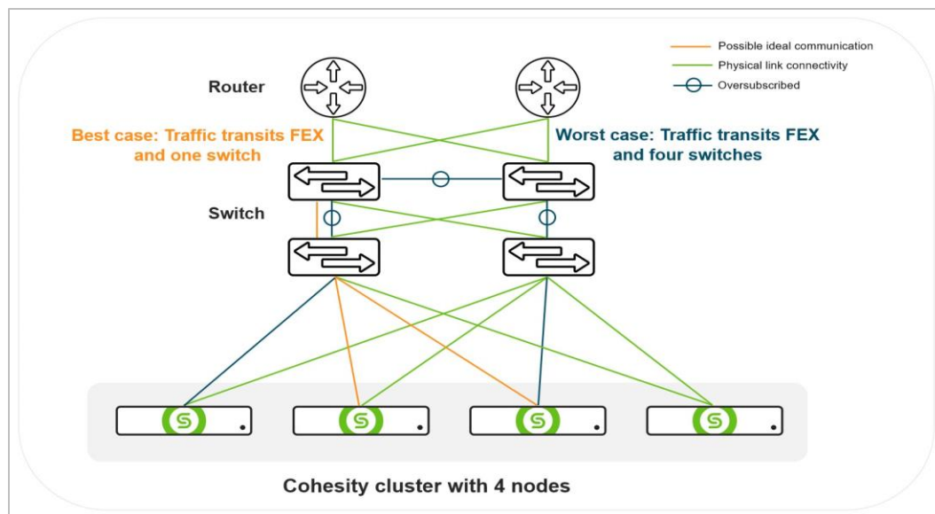
Figure 4: Cohesity on a Cisco FEX Topology
