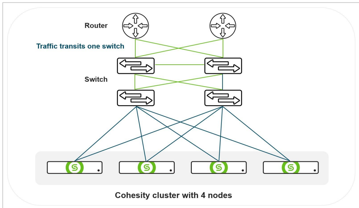
Figure 5: Cohesity on a Layered Bond Mode 4 (LACP) Topology
