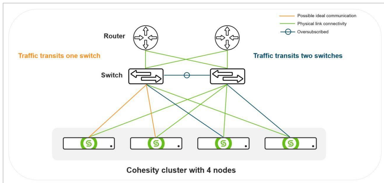
Figure 2: Cohesity on a Standard Topology
